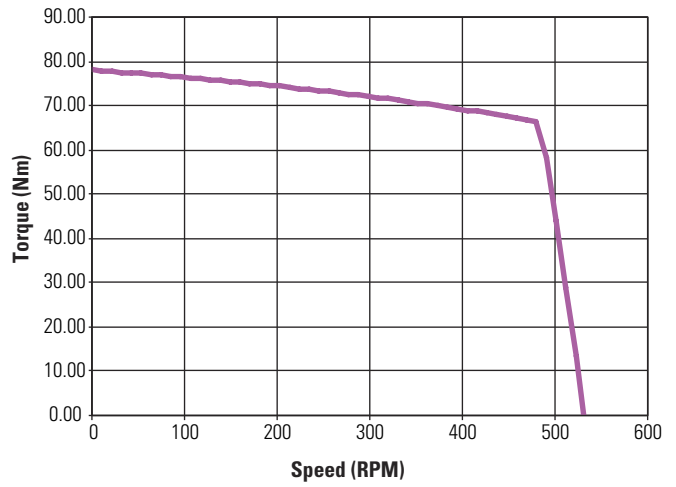
KBM(S)-79X02 ContinuousTorque
