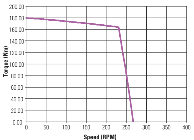
KBM(S)-79X04 ContinuousTorque
