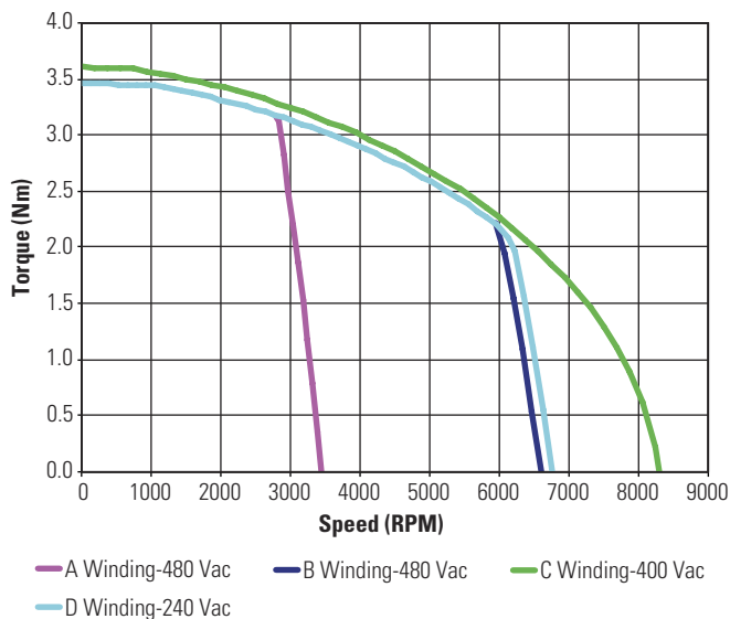
KBM(S)-17X02 Continuous Torque
