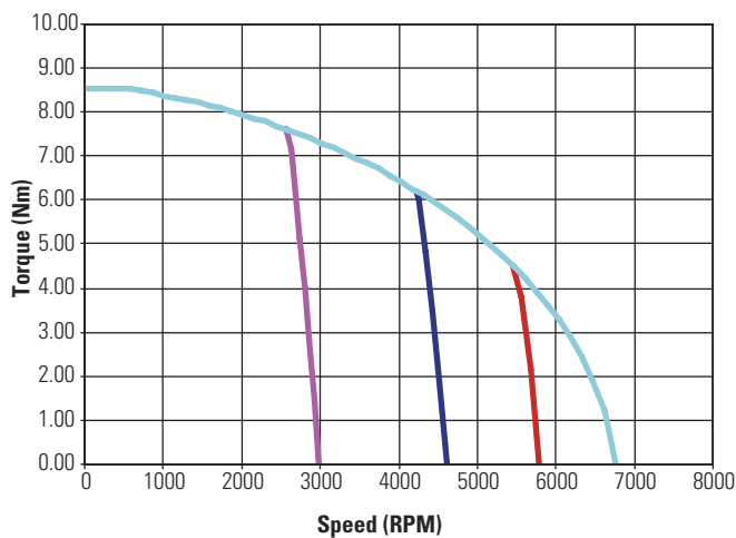
KBM(S)-25X02 ContinuousTorque
