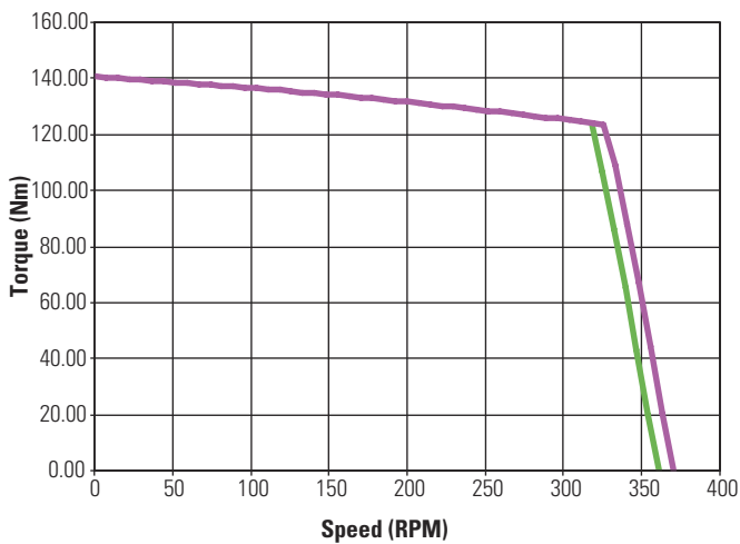
KBM(S)-79X03 ContinuousTorque
