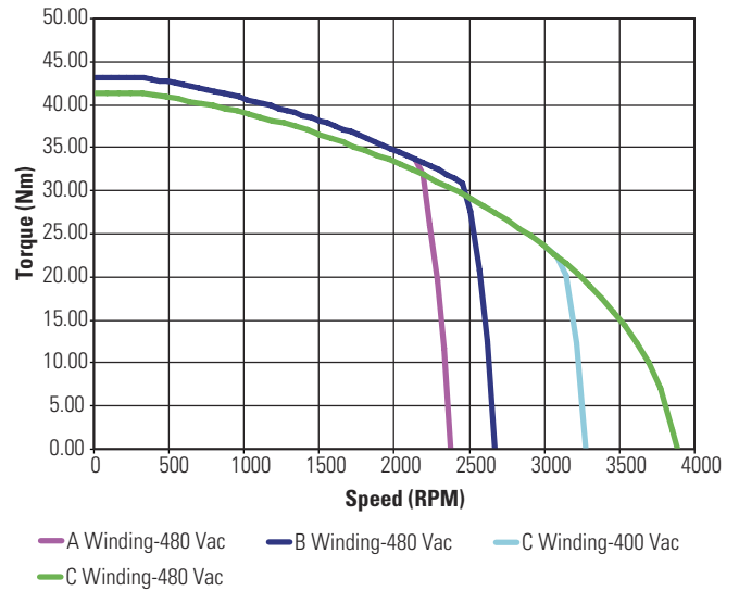
KBM(S)-45X02 Continuous Torque
