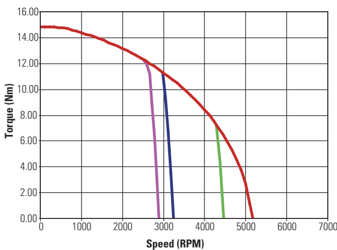
KBM(S)-25X04 ContinuousTorque
