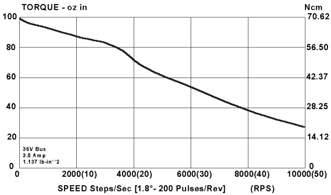
KML062F13 MOTOR
