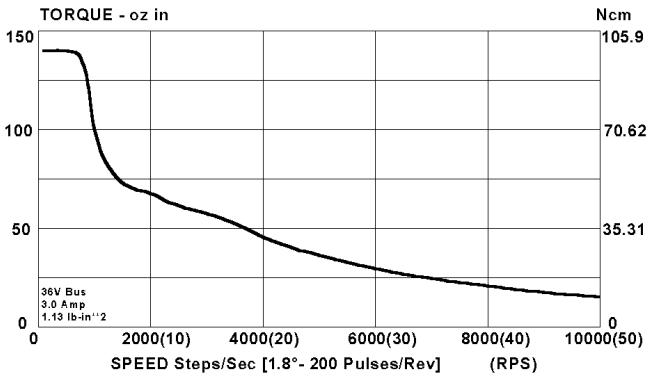
KML061F05 MOTOR
