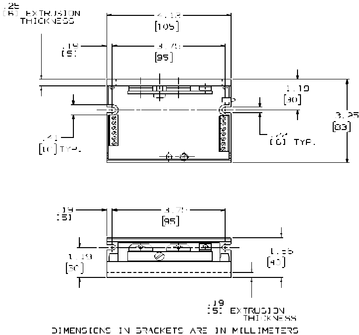
Figure 3.1, Mounting Diagram
